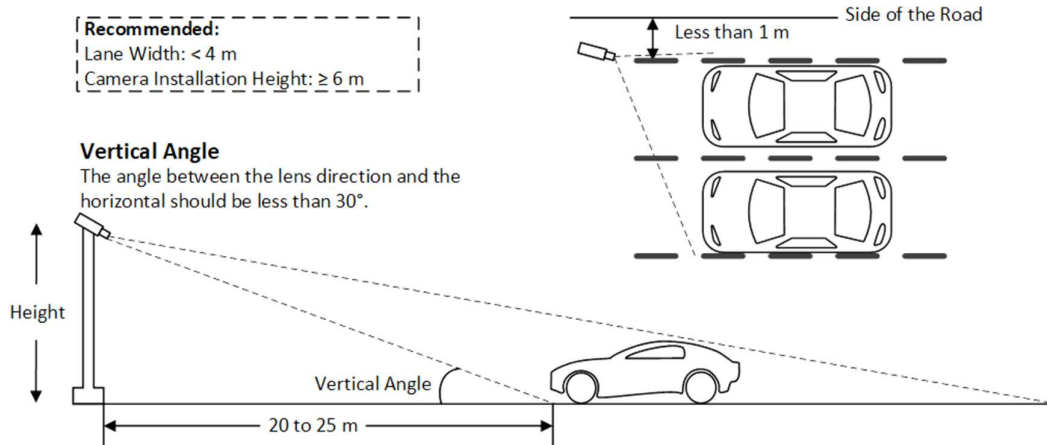
Figure 1-4 City Street Installation Diagram (On the Side of the Gantry)
