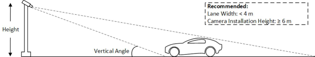
Figure 1-1 Installation Diagram
