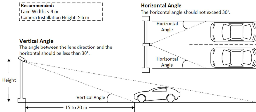
Figure 1-3 City Street Installation Diagram (In the Middle of the Gantry)
